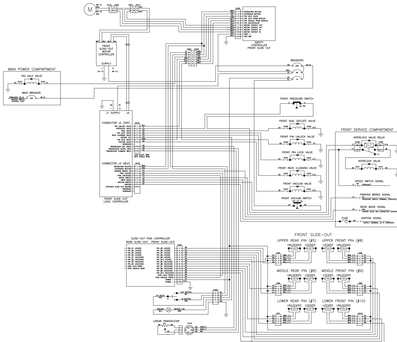
XL2 SINGLE SLIDE-OUT ELECTRIC DIAGRAM (RETROFIT) EFFECTIVE FROM SERIAL NUMBER Y-7450 TO 1-7718 AND FROM 1-7724 TO 1-7773 (ALL WIRES ARE 18 AWG EXCEPT WHEN SPECIFIED)
